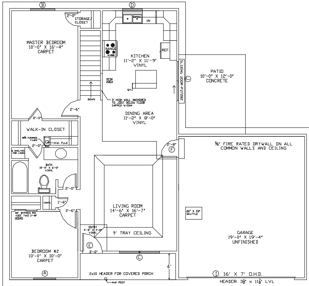
FIRST FLOOR PLAN - 1045 SF
