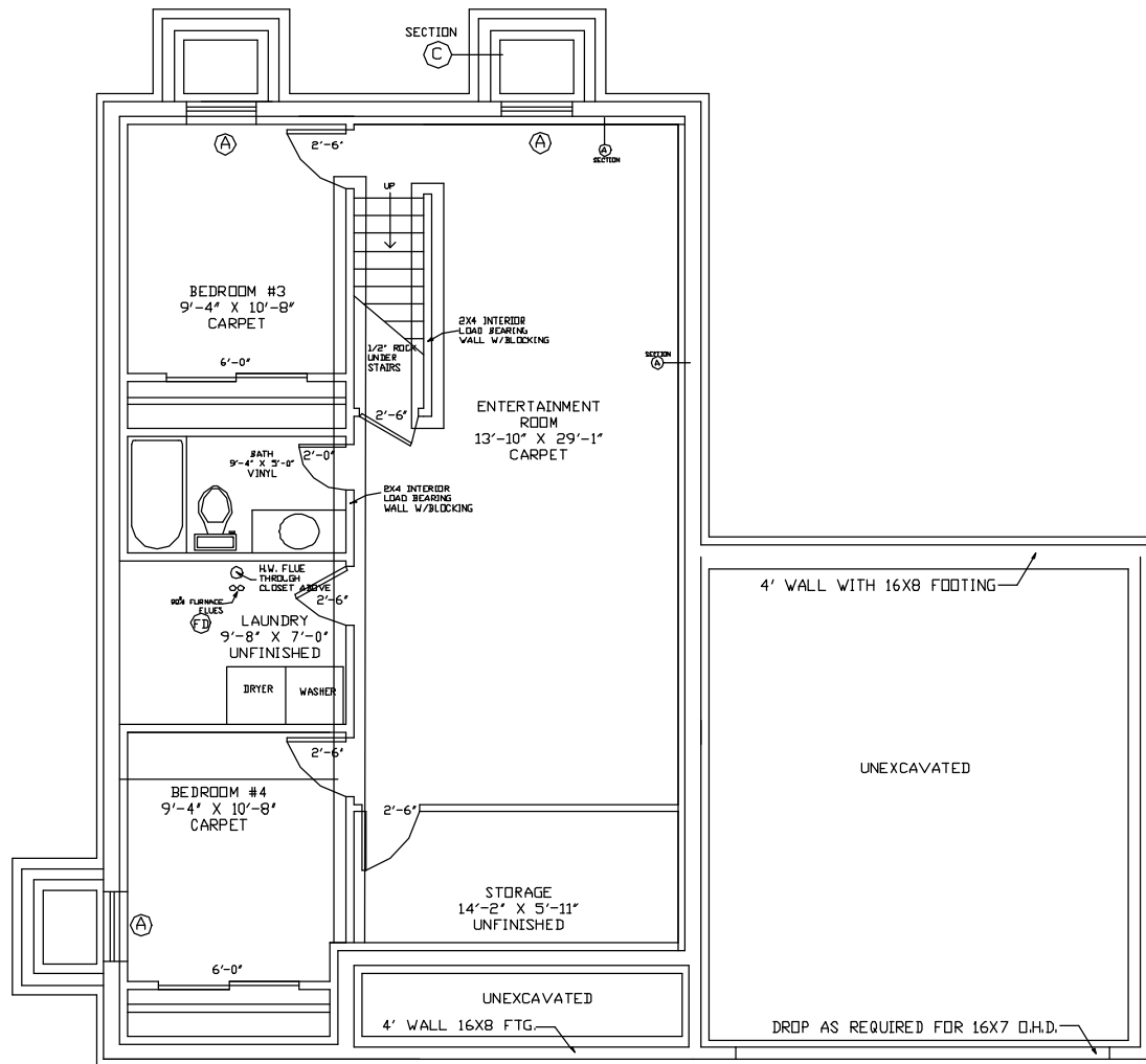
FOUNDATION PLAN - 837 SF-FINISHED
